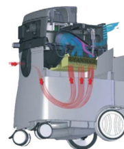
Air cycle during normal operation
